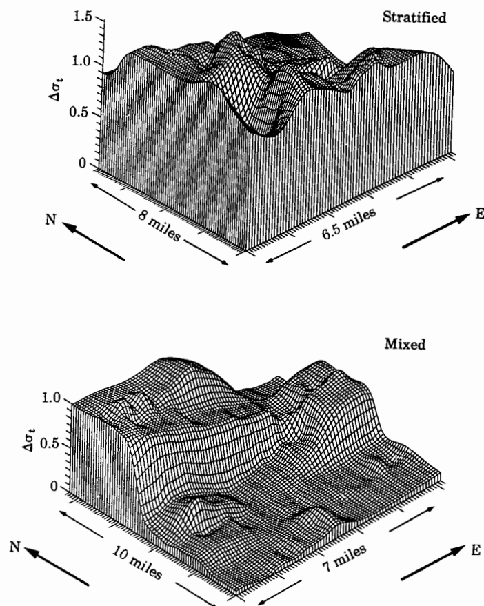
Figure 2. Three-dimensional representation of the density field (surface-to-bottom density difference) at the mixed and stratified sampling sites on the June 1990 cruise.
