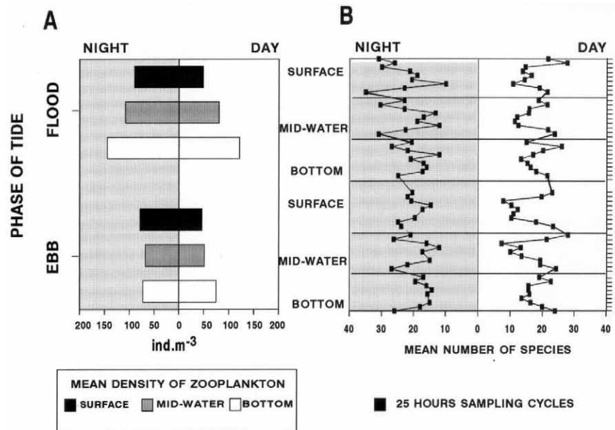
FIG. 3. – Mean density of zooplankton (A) and mean number of species (B), during flood and ebbs, in the day and night periods, at the three depths. Concentrations (ind. m -3 ) are represented by horizontal bars. Shaded area: night.
