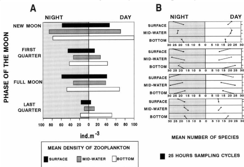
FIG. 4. – Mean density of zooplankton (A) and mean number of species (B), during the phases of the moon, in the day and night periods, at the three depths. Concentrations (ind. m -3 ) are represented by horizontal bars. Shaded area: night.
