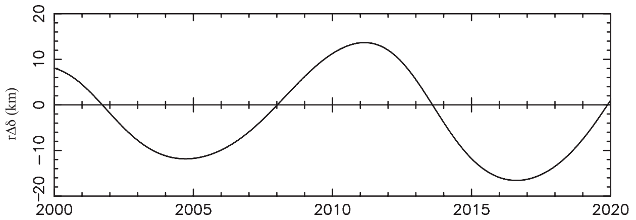
Figure 10. Difference in position of Jupiter with respect to the Sun in direction of increasing declination from DE435 compared with DE434.
