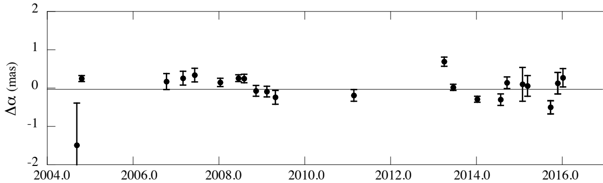
Figure 7: Residuals of VLBA right ascension measurements Saturn updated after creation of DE435.
