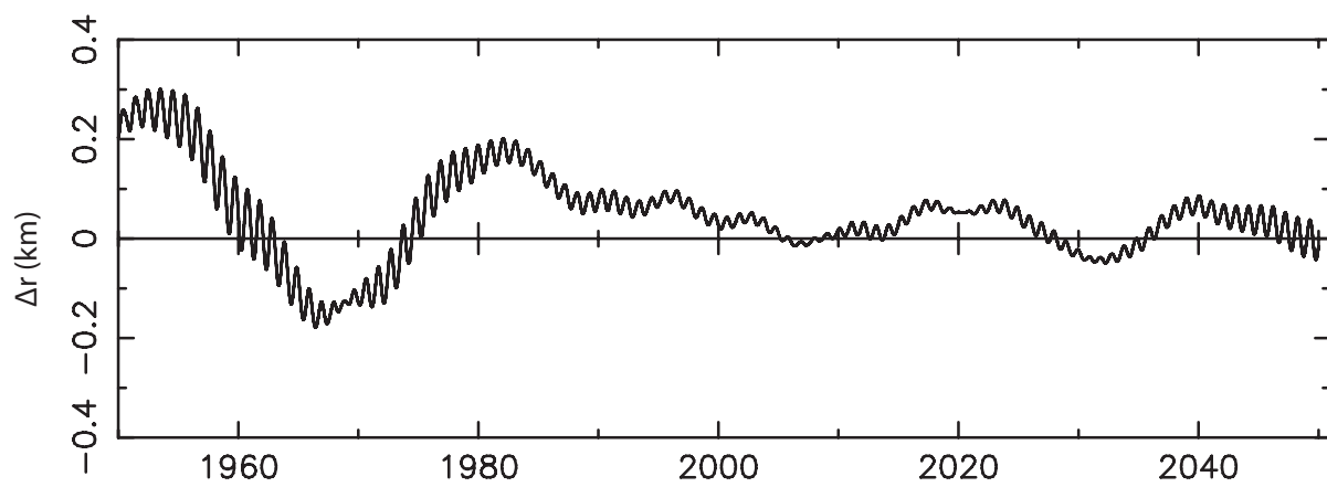
Figure 6. Difference in distance of Saturn to Earth from DE435 compared with DE430.
