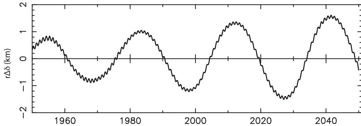
Figure 5. Difference in position of Saturn relative to Earth in direction of increasing declination from DE435 compared with DE430.
