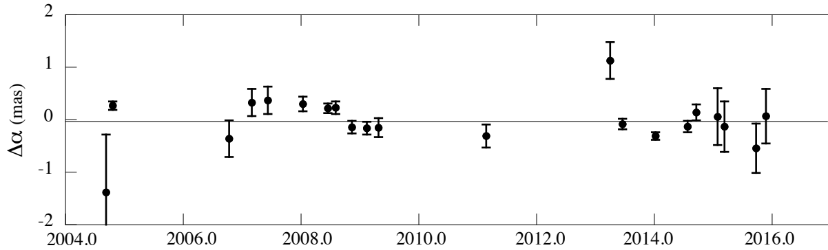
Figure 2: Residuals of VLBA right ascension measurements Saturn used for DE435.
