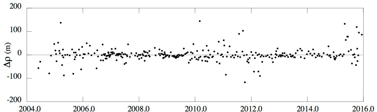
Figure 1: Residuals of distance of the Saturn system barycenter from Earth on DE435 from Cassini spacecraft range measurements and orbits estimated from Doppler data.
