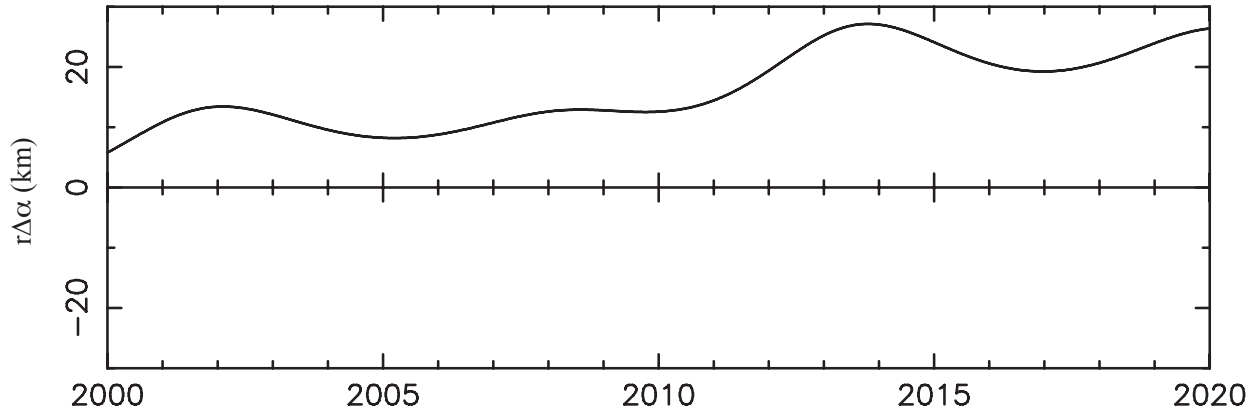
Figure 9. Difference in position of Jupiter with respect to the Sun in direction of increasing right ascension from DE435 compared with DE434.
