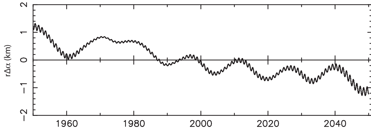
Figure 4. Difference in position of Saturn relative to Earth in direction of increasing right ascension from DE435 compared with DE430.
