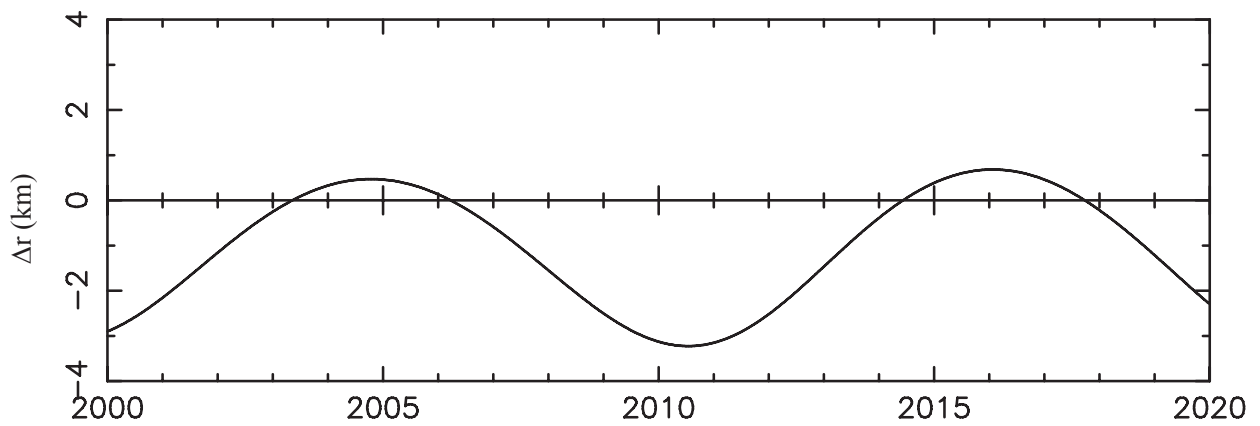
Figure 11. Difference in distance of Jupiter with respect to the Sun from DE435 compared with DE434.
